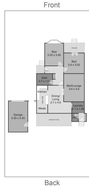
Site Plan
