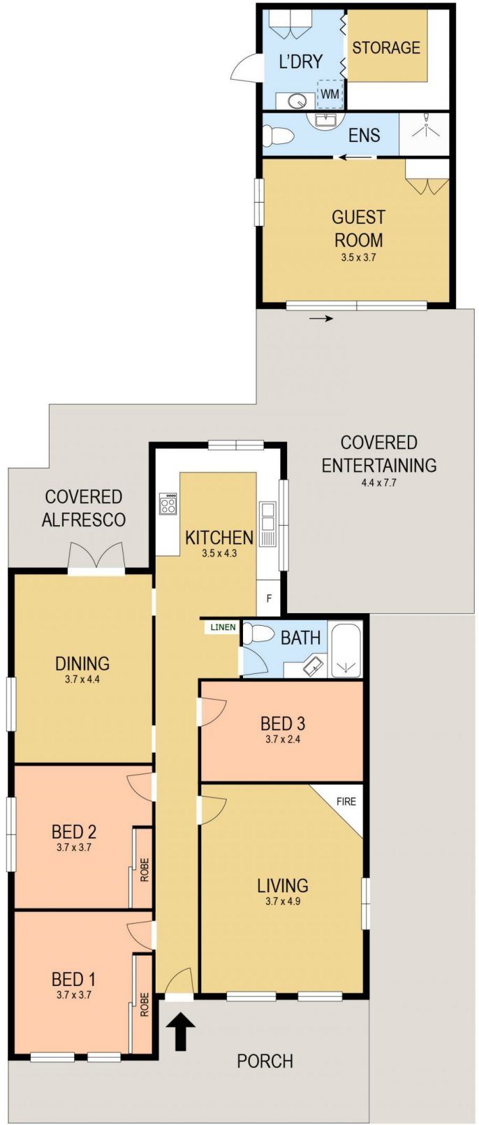
FLOOR PLAN
