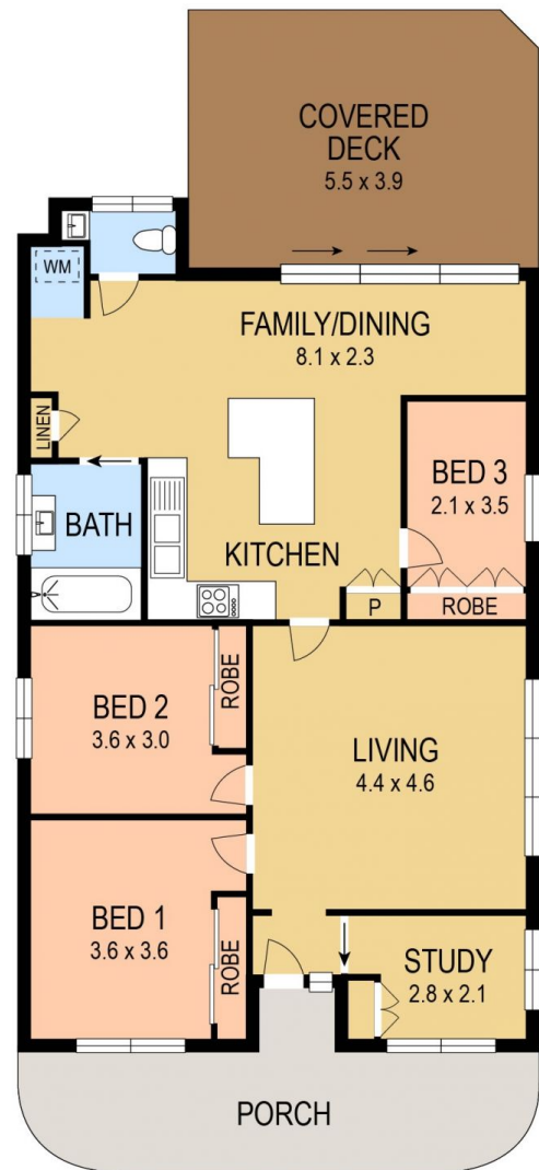
FLOOR PLAN
