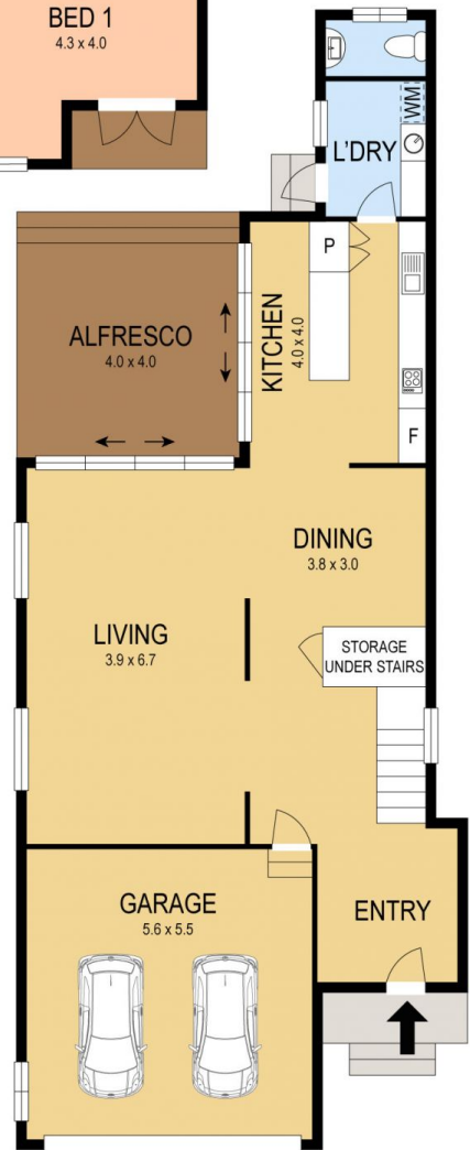
LOWER FLOOR
