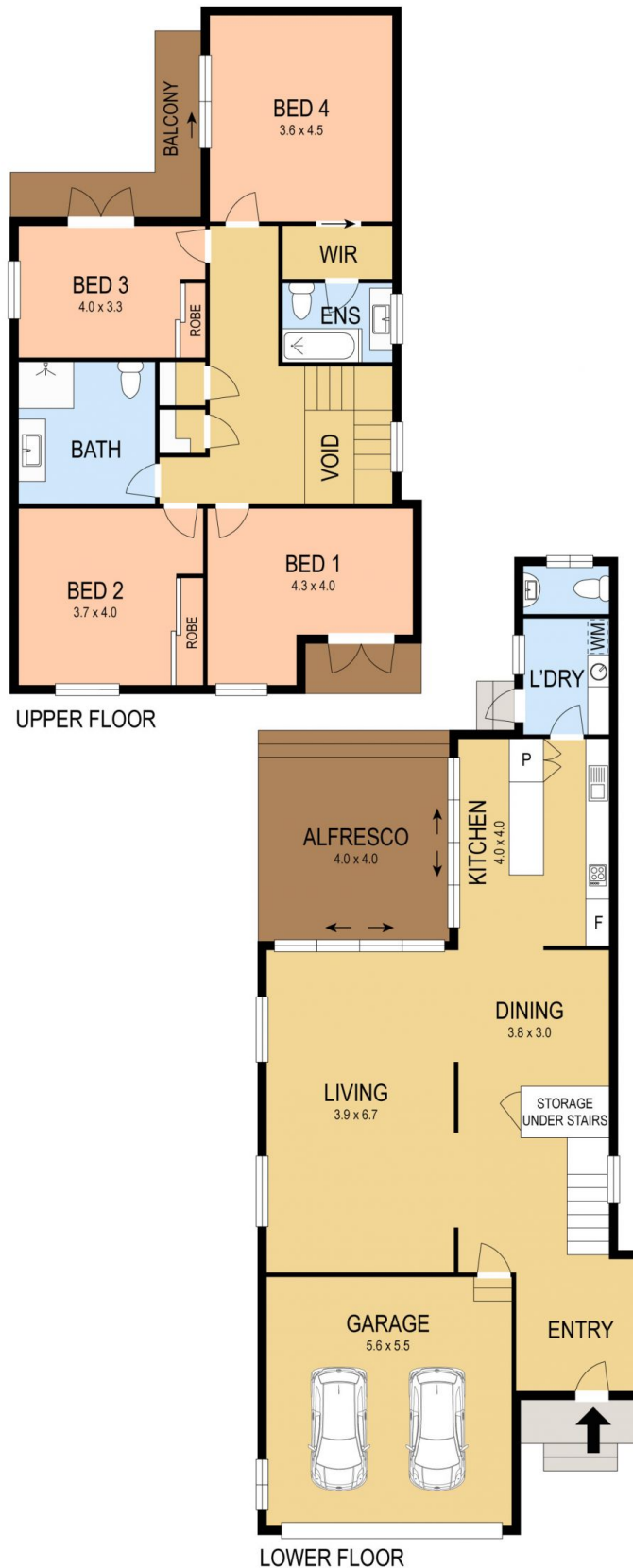
FLOOR PLAN
