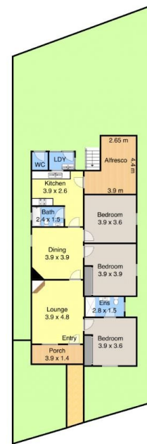
Site Plan
