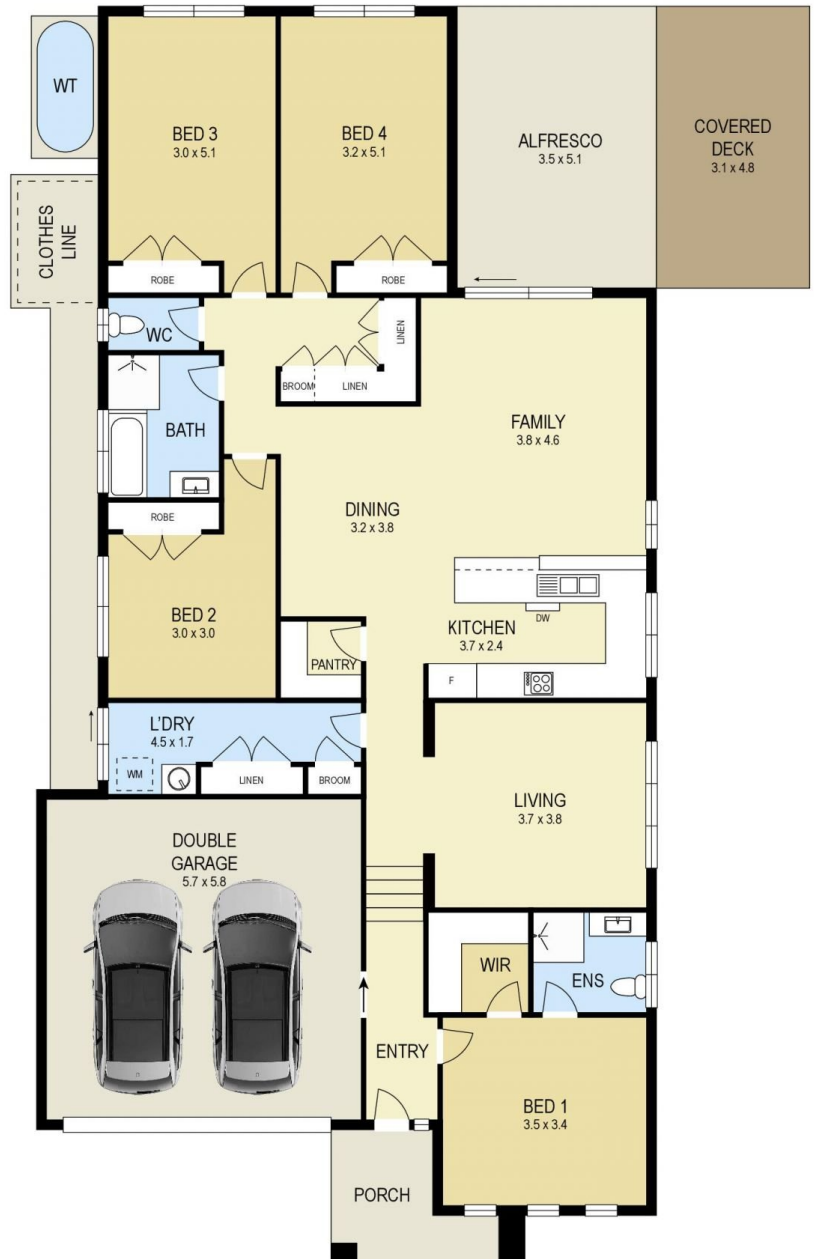
FLOOR PLAN
