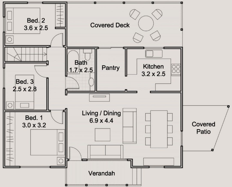
Upper Floor Plan Residence Area: 112 sqm
