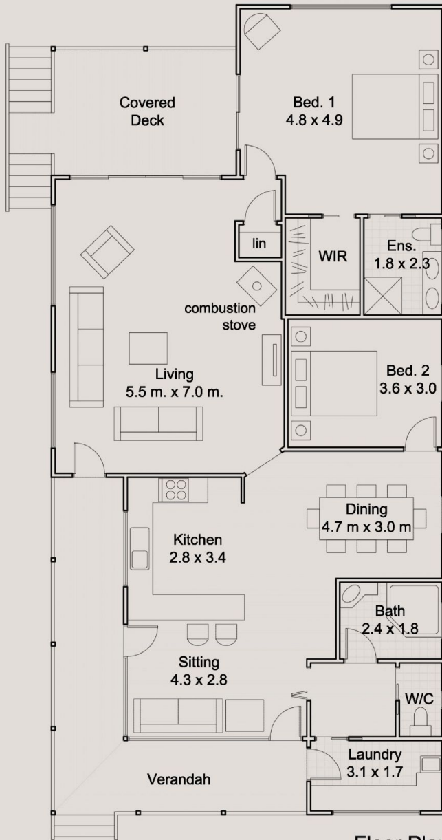
Floor Plan Total Residence Area: 256 sqm
